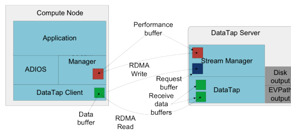
Figure 6.3: DataTap architecture
